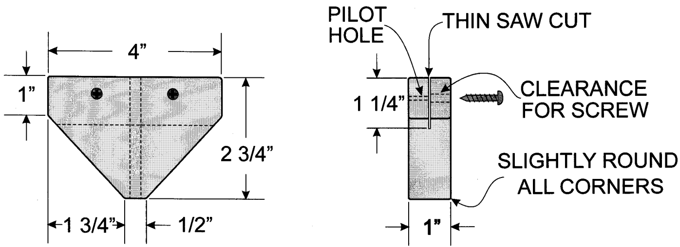
BEVEL BLOCK
