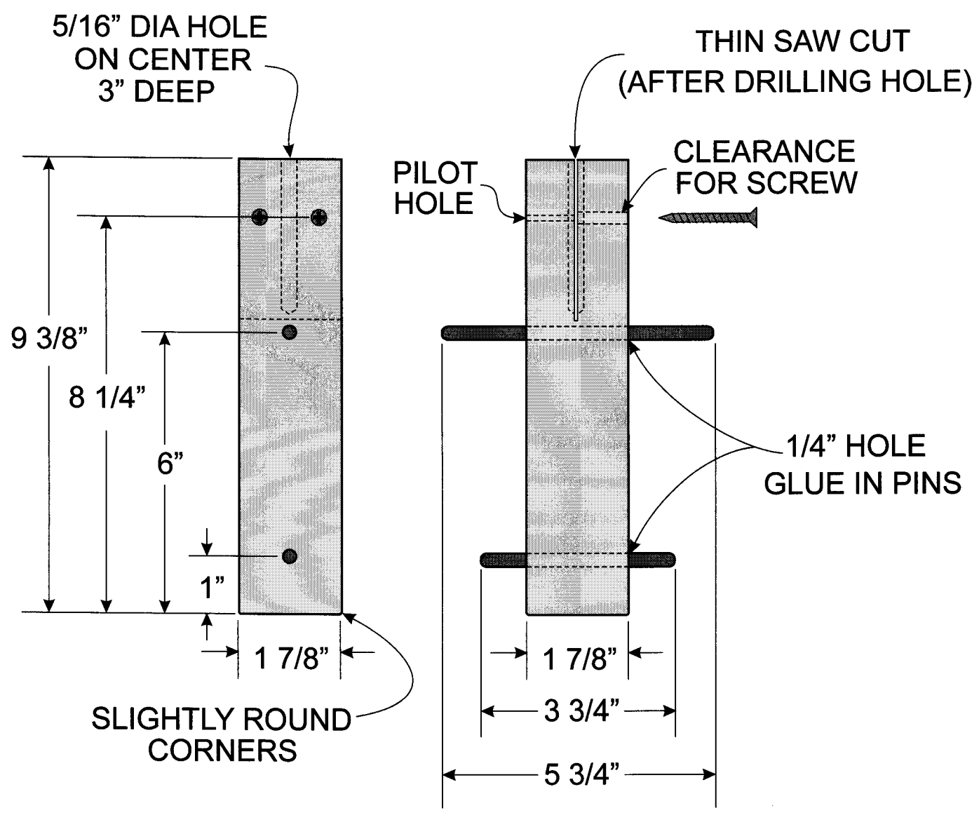
PIN BLOCK
